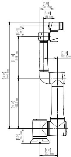
JAKA Zu 30 Outline Dimension
