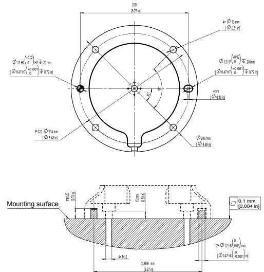
JAKA Zu 30 Base Dimension
