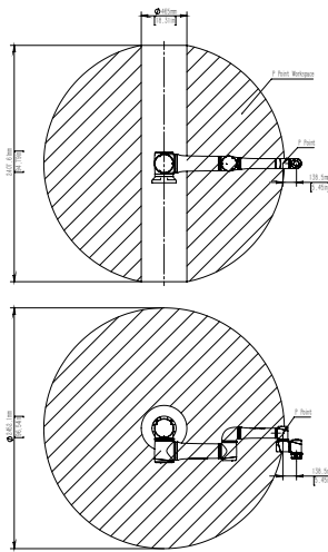
JAKA Zu 30 Workspace Dimension
